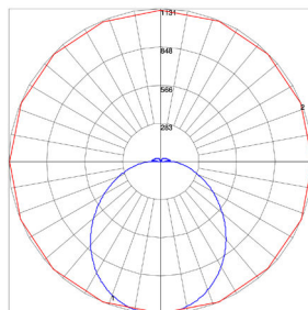
Maximum Candela = 1131 Located At Horizontal Angle = 225, Vertical Angle = 2.5 #1 - Vertical Plane Through Horizontal Angles (225 - 45) Through Max. Cd #2 - Horizontal Cone Through Vertical Angle (2.5) Through Max. Cd TSS 4 30/40/50 G1 FSK Lumen setting (30 - 3120 LM) CCT setting 3500K Wattage (24W)
