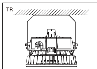
Trunnion Mount
