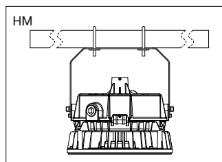
Hoop Clamp Mount
