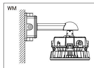
Wall Mount
