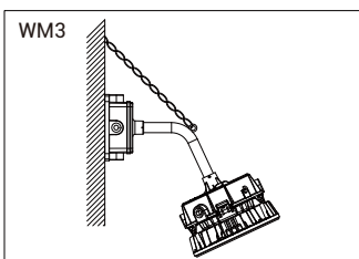
Wall Mount (115° Pole)
