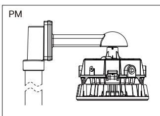
Round Pole Mount
