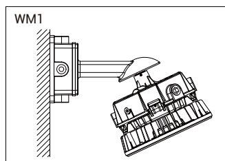
Wall Mount (115°)
